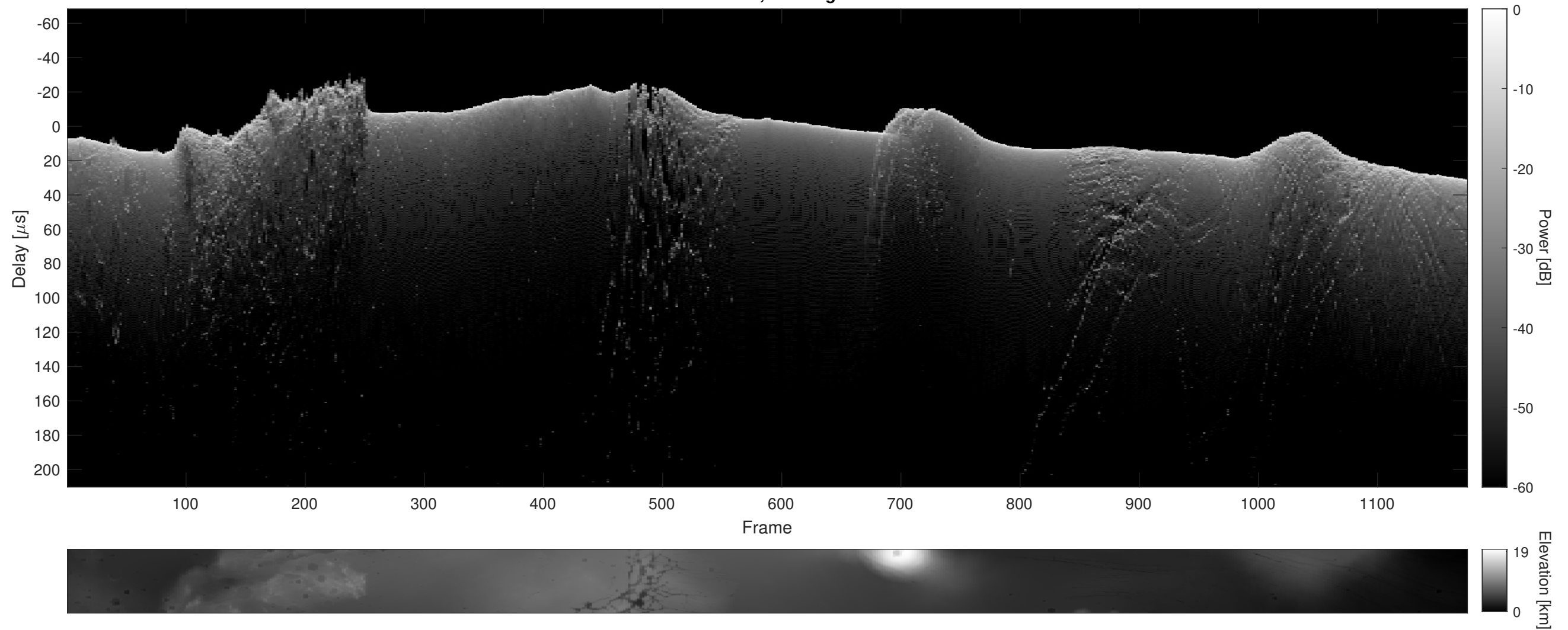
Orbit 10300, Cluttergram
