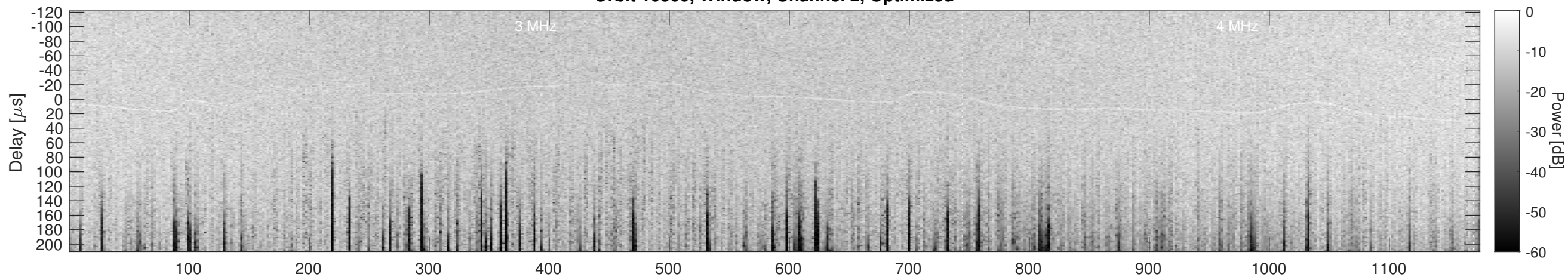
Orbit 10300, Cluttergram
