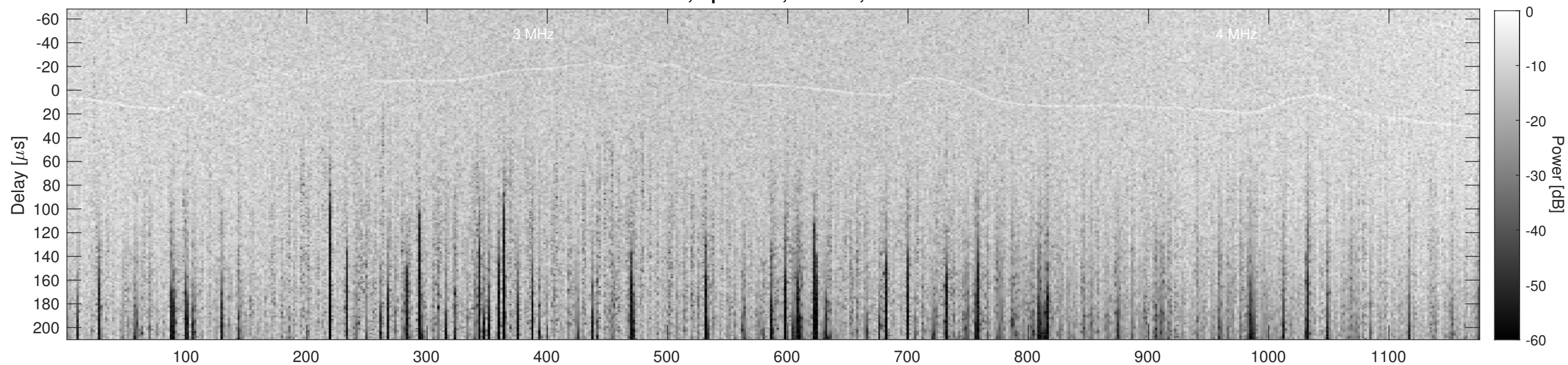
Orbit 10300, Cluttergram
