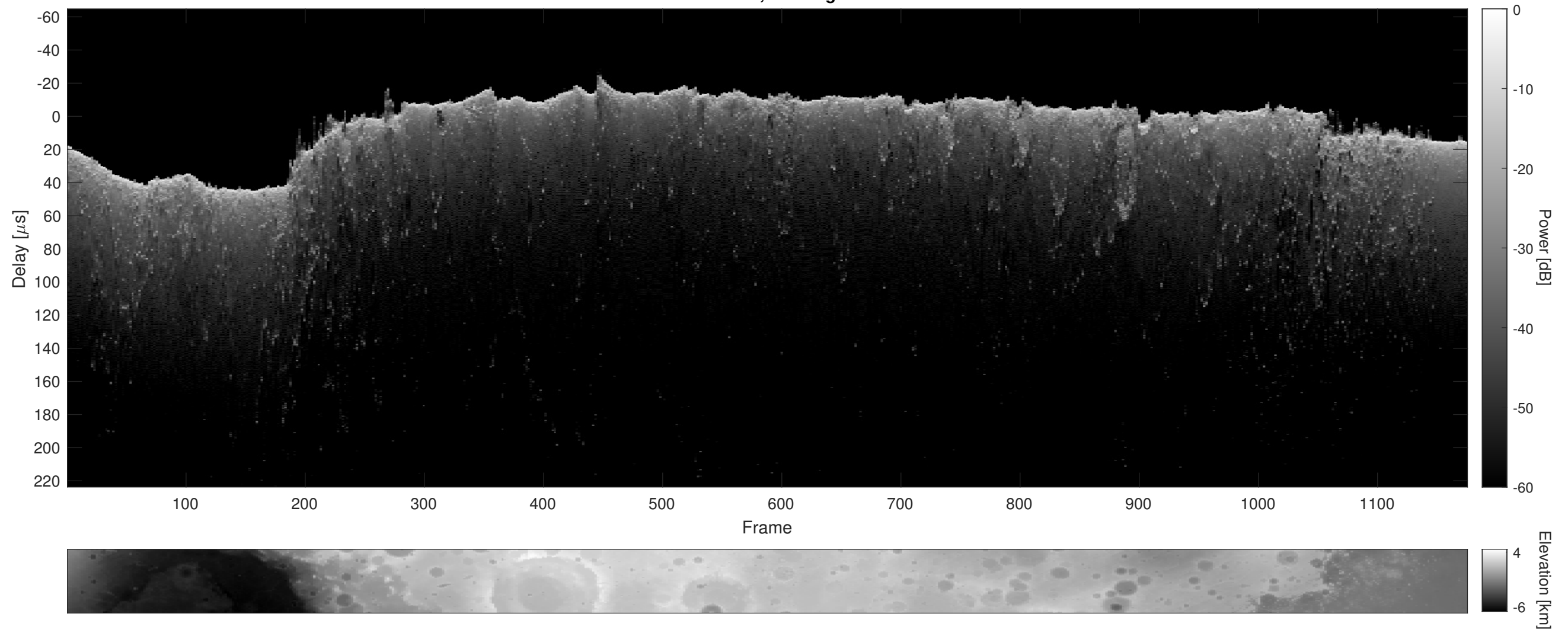
Orbit 10302, Cluttergram
