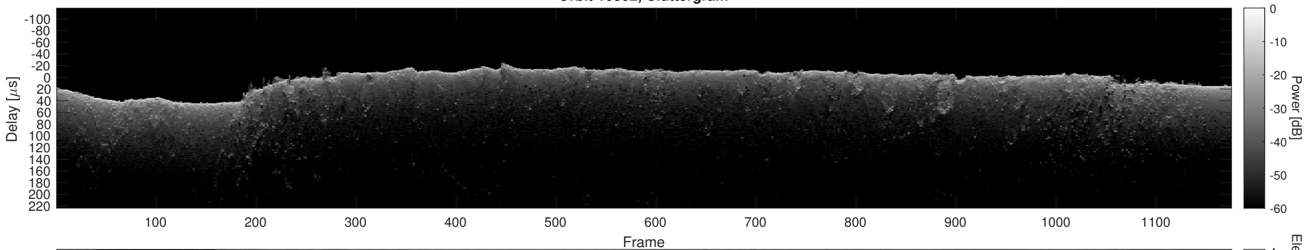
Orbit 10302, Cluttergram
