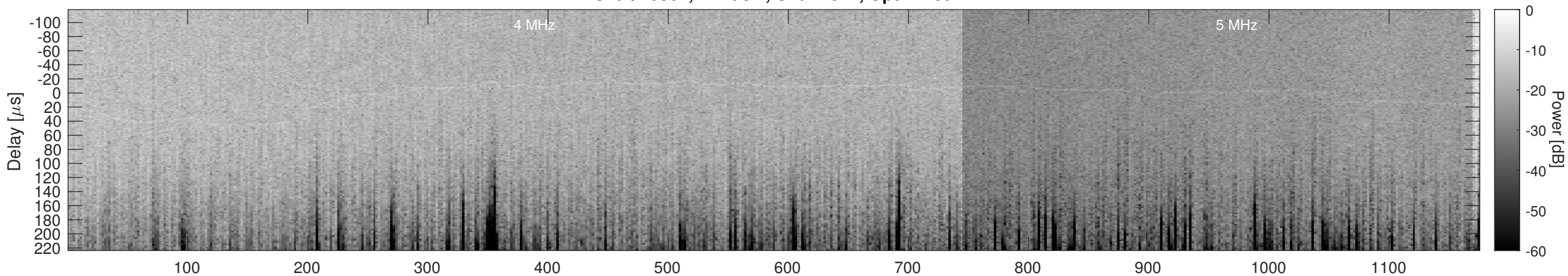
Orbit 10302, Cluttergram
