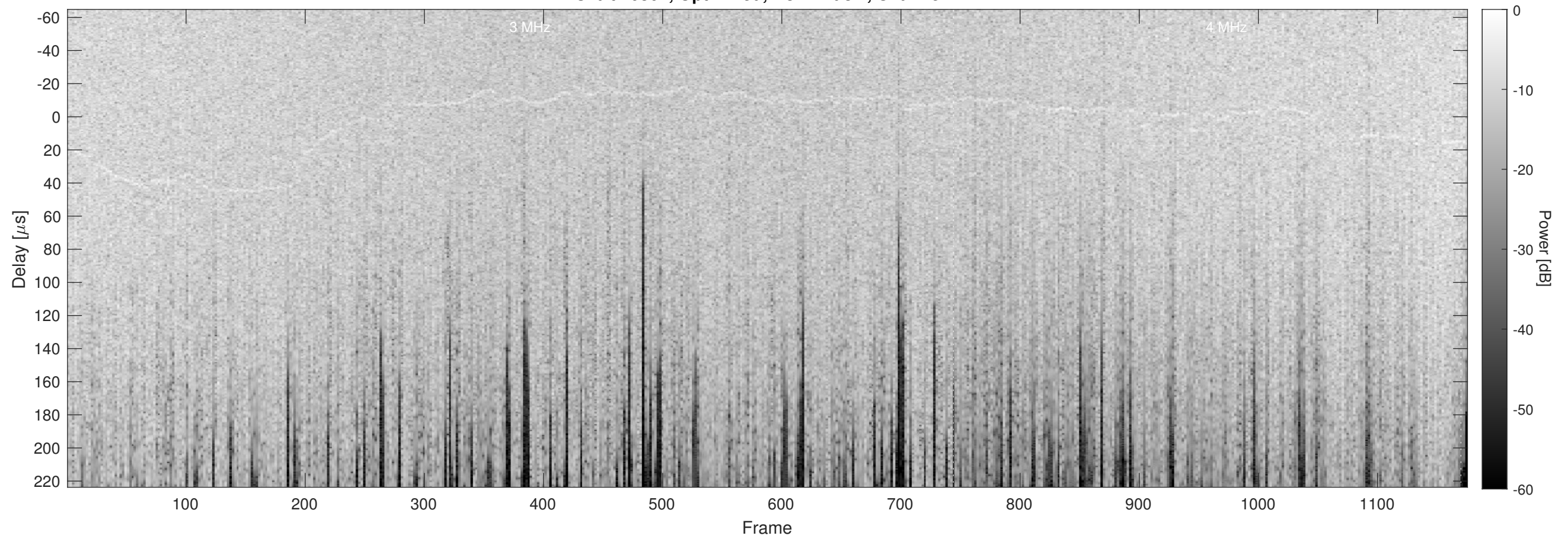
Orbit 10302, Optimized, No Window, Channel 2
