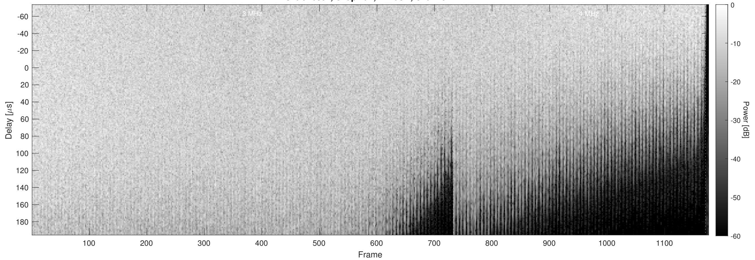
Orbit 10304, Chapman, Window, Channel 2
