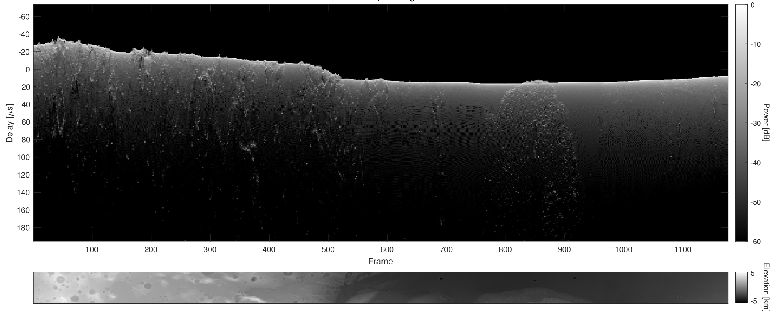
Orbit 10304, Cluttergram
