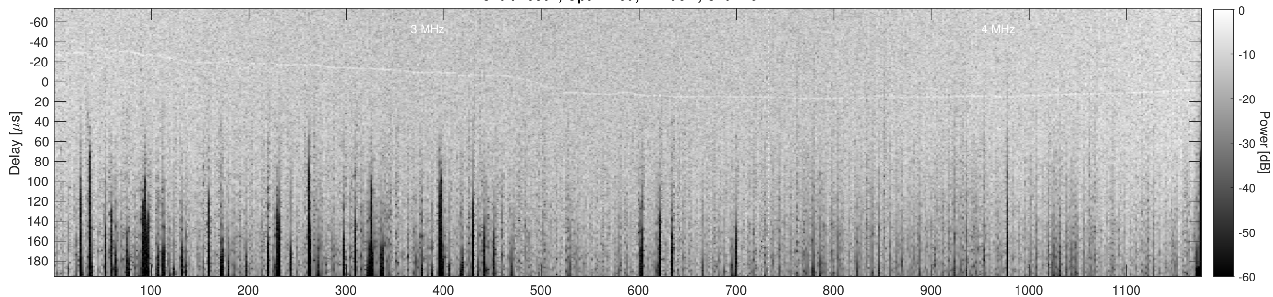
Orbit 10304, Cluttergram
