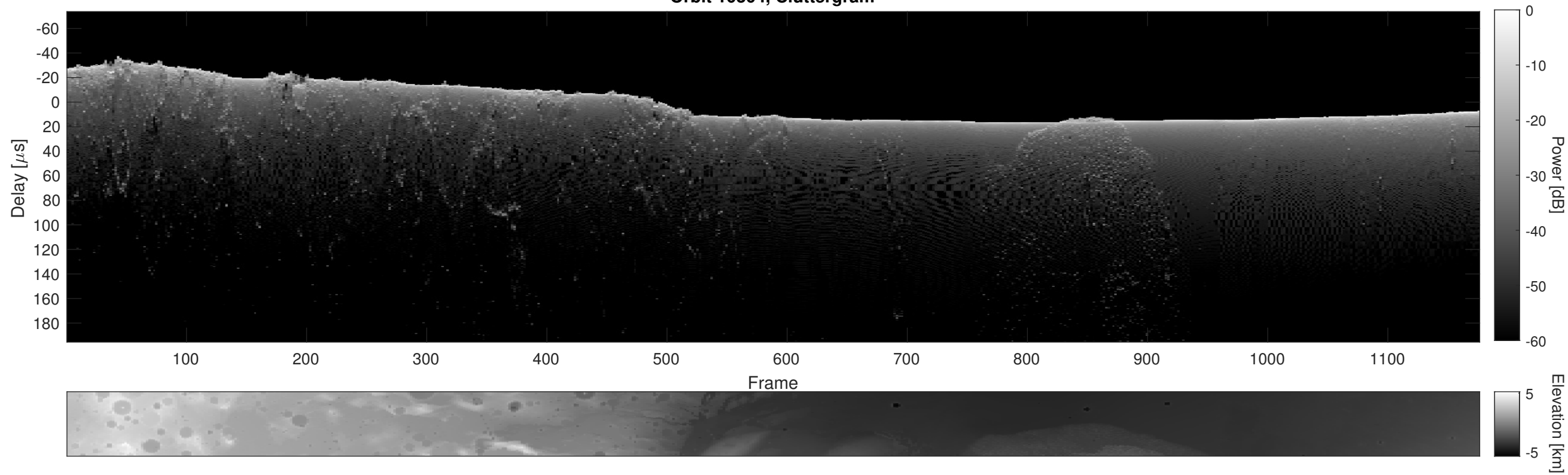
Orbit 10304, Cluttergram
