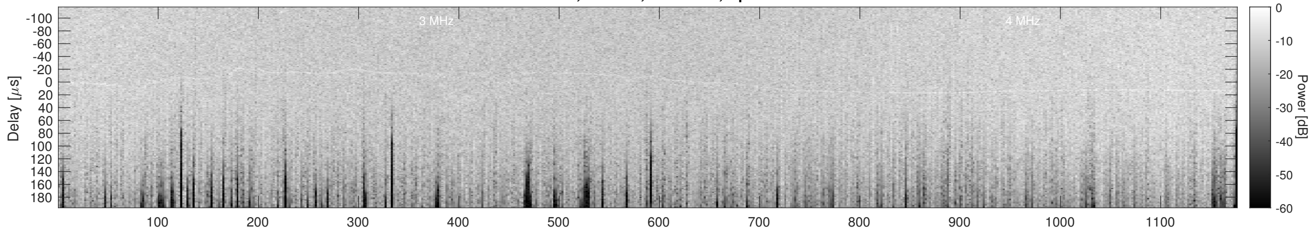
Orbit 10310, Cluttergram
