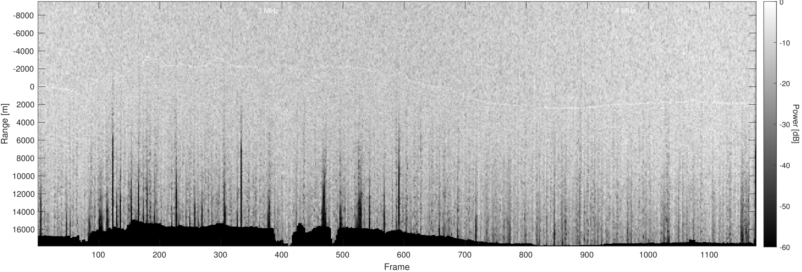
Orbit 10310, Optimized, Window, Depth-Corrected, Channel 2
