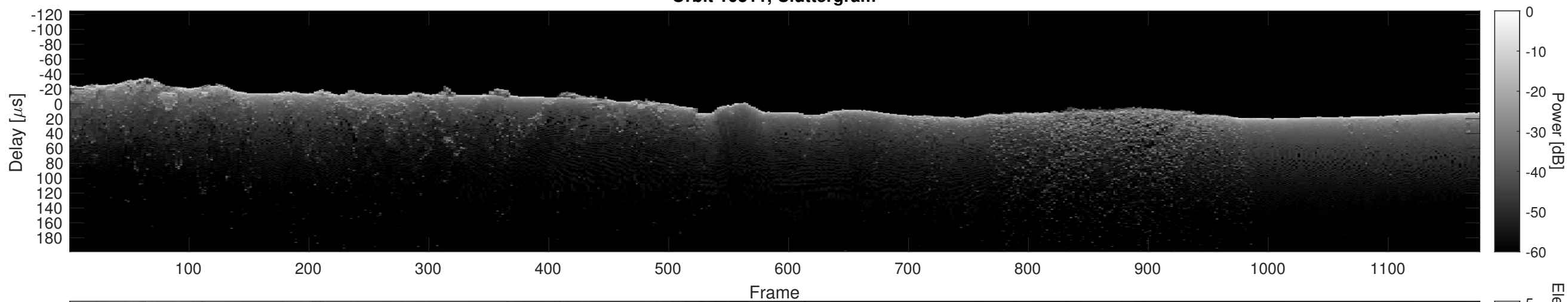
Orbit 10311, Cluttergram
