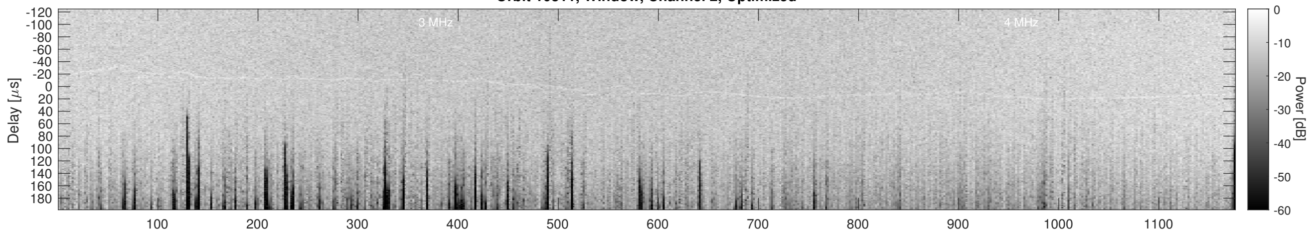
Orbit 10311, Cluttergram
