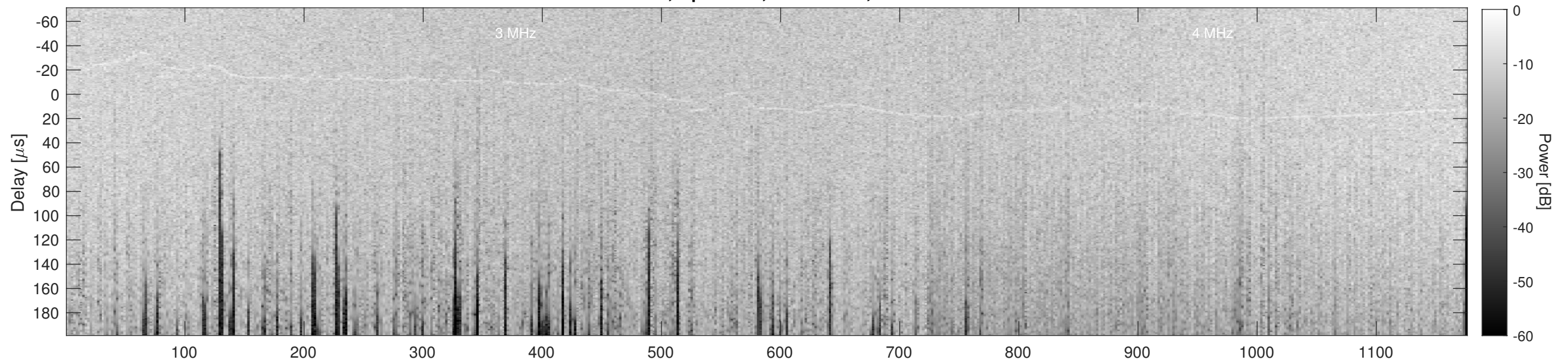
Orbit 10311, Cluttergram
