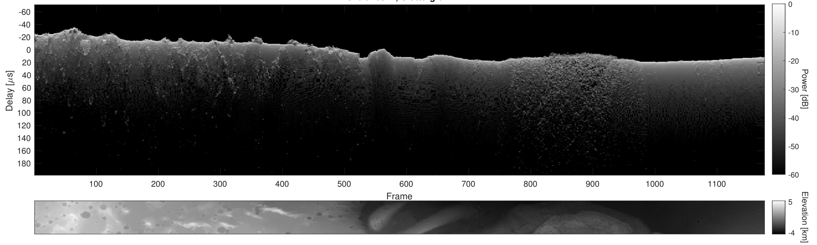
Orbit 10311, Cluttergram
