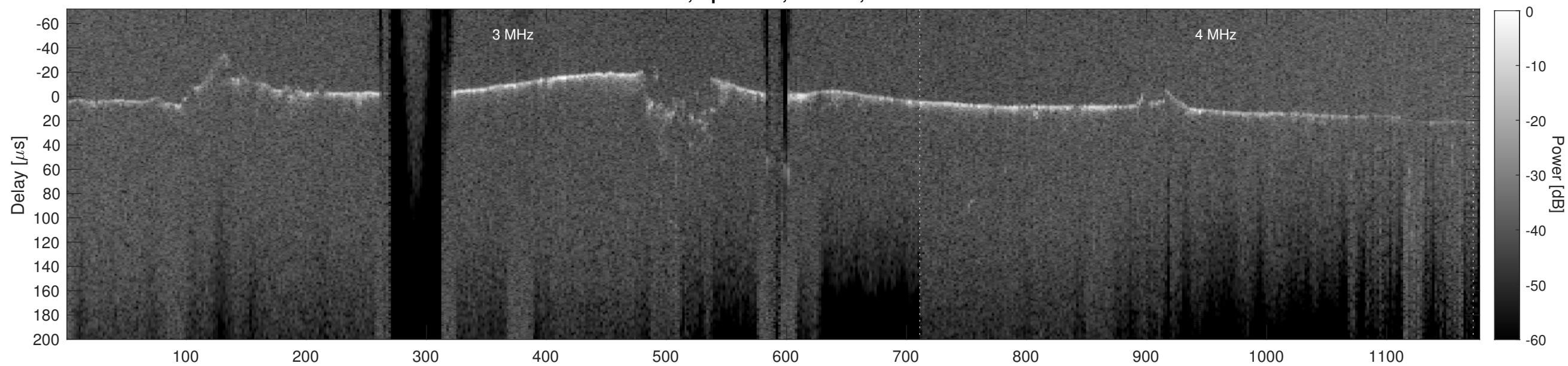
Orbit 10314, Cluttergram
