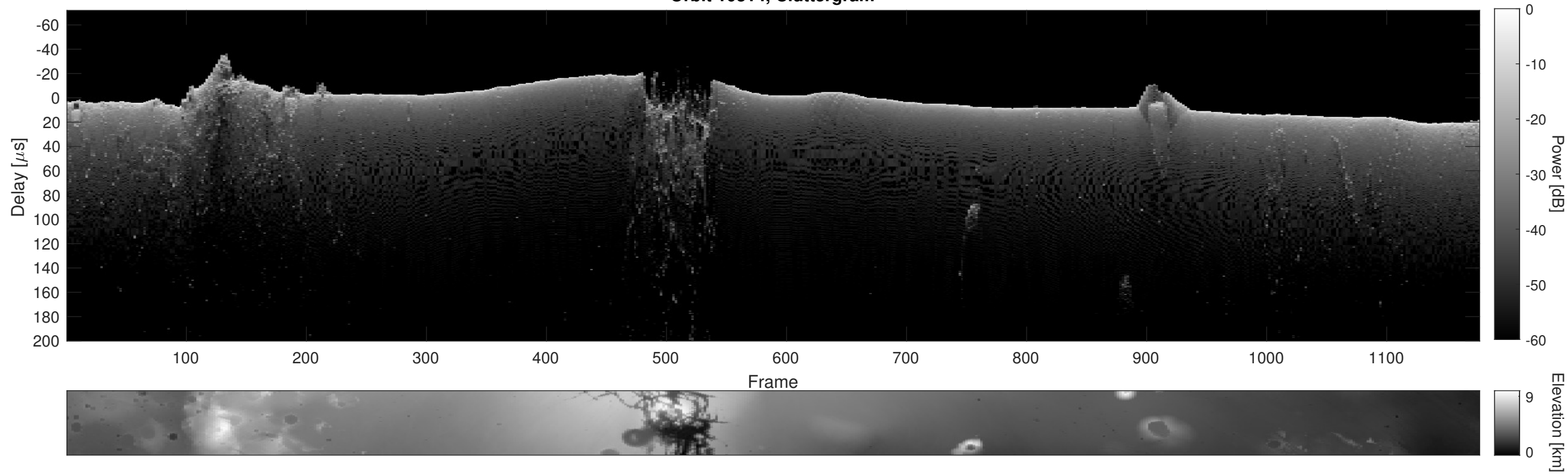
Orbit 10314, Cluttergram
