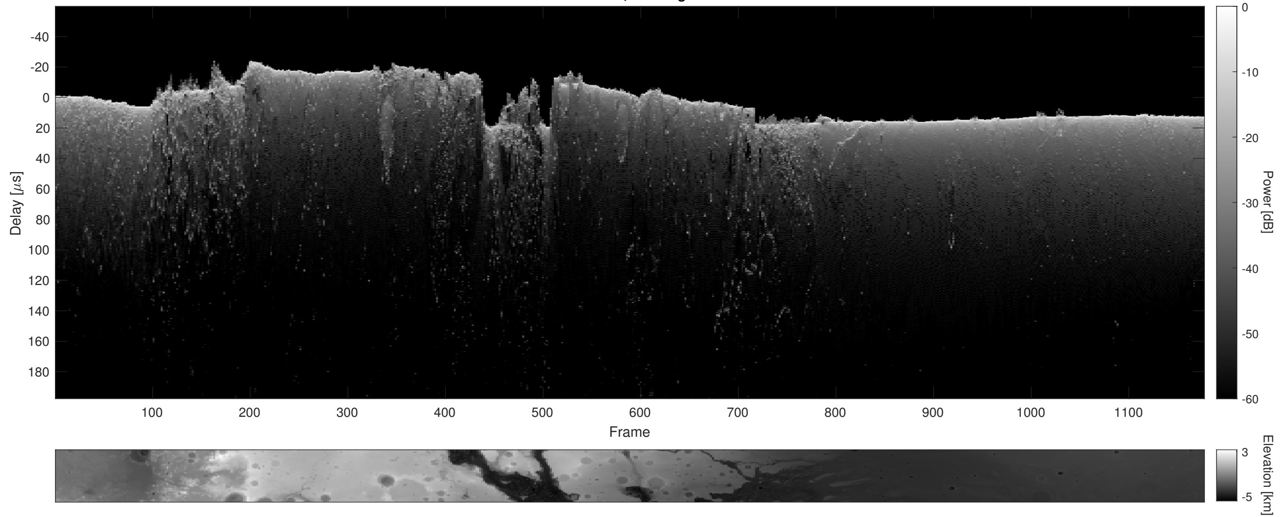
Orbit 10317, Cluttergram
