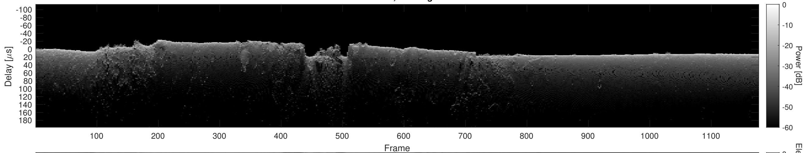
Orbit 10317, Cluttergram
