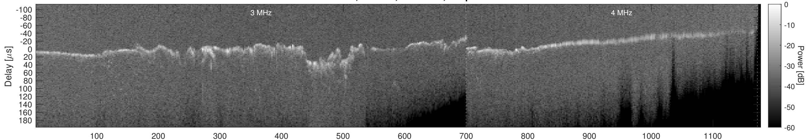
Orbit 10317, Window, Channel 2, Optimized
