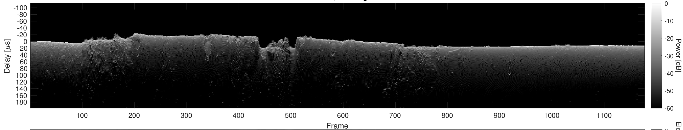
Orbit 10317, Cluttergram
