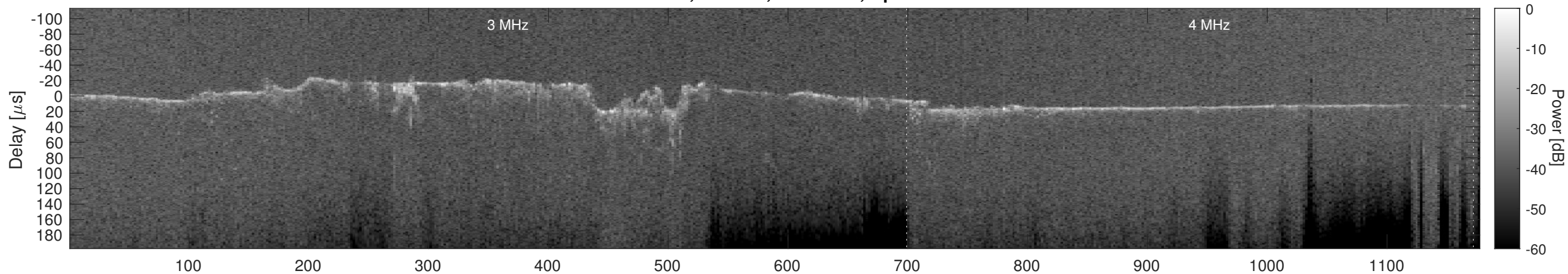
Orbit 10317, Cluttergram
