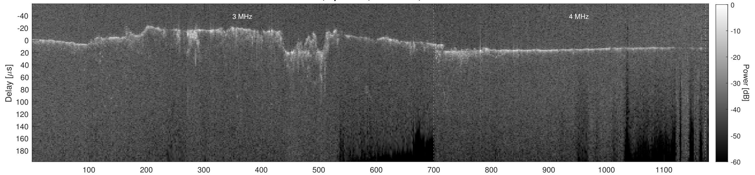
Orbit 10317, Cluttergram
