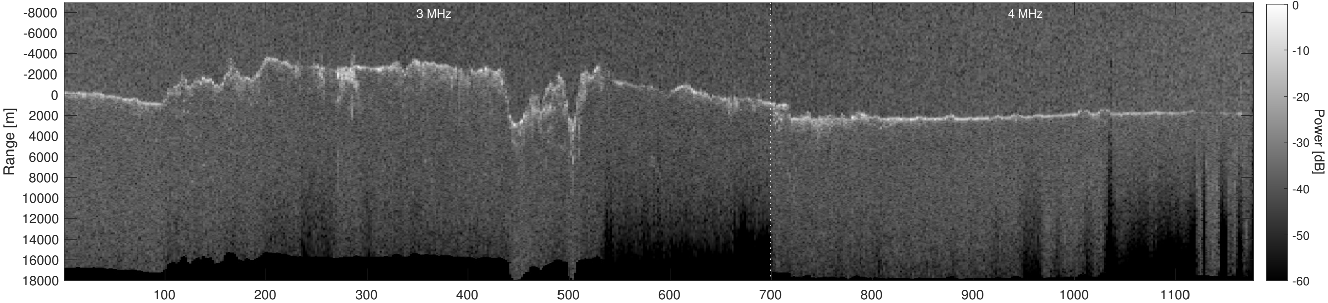
Orbit 10317, Depth-Corrected Cluttergram
