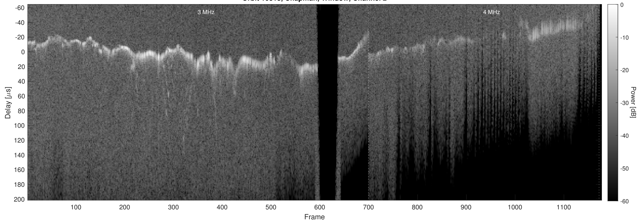
Orbit 10318, Chapman, Window, Channel 2
