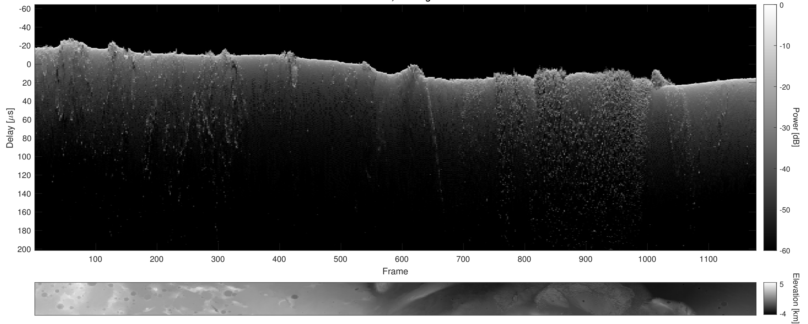
Orbit 10318, Cluttergram
