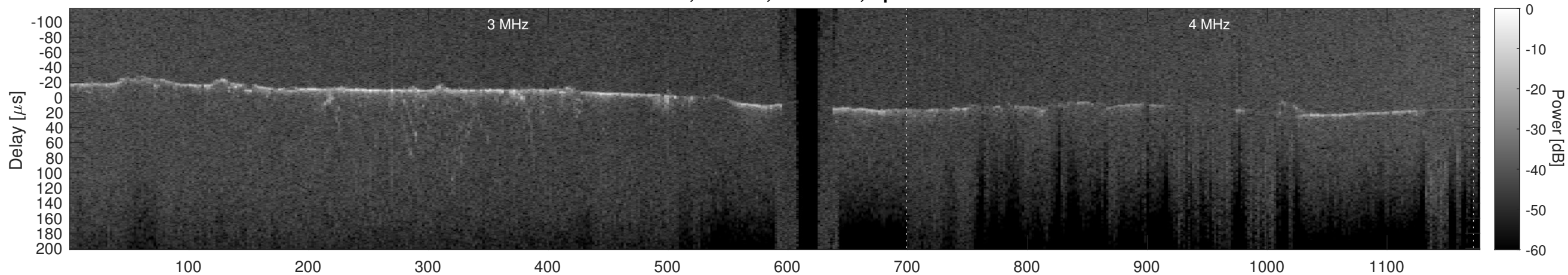
Orbit 10318, Cluttergram
