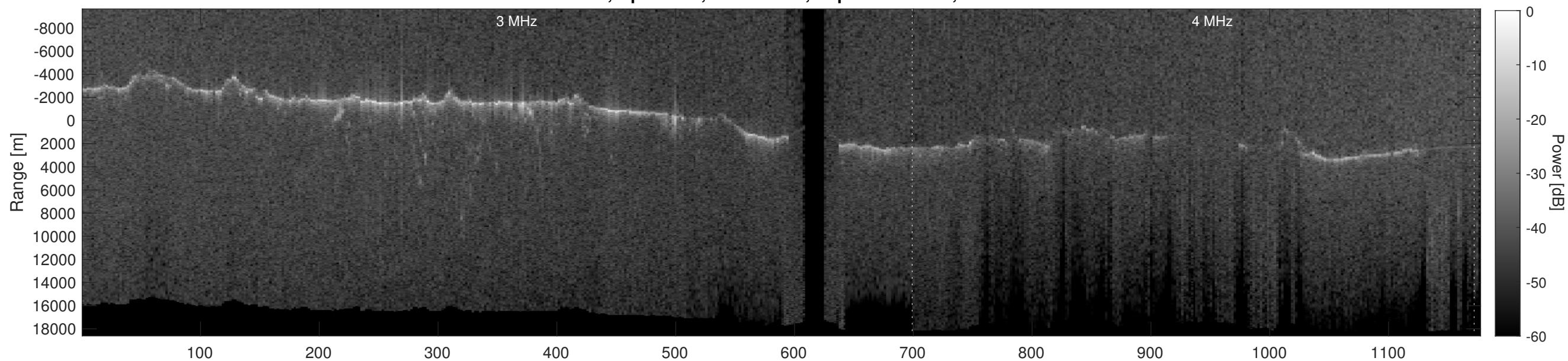
Orbit 10318, Depth-Corrected Cluttergram
