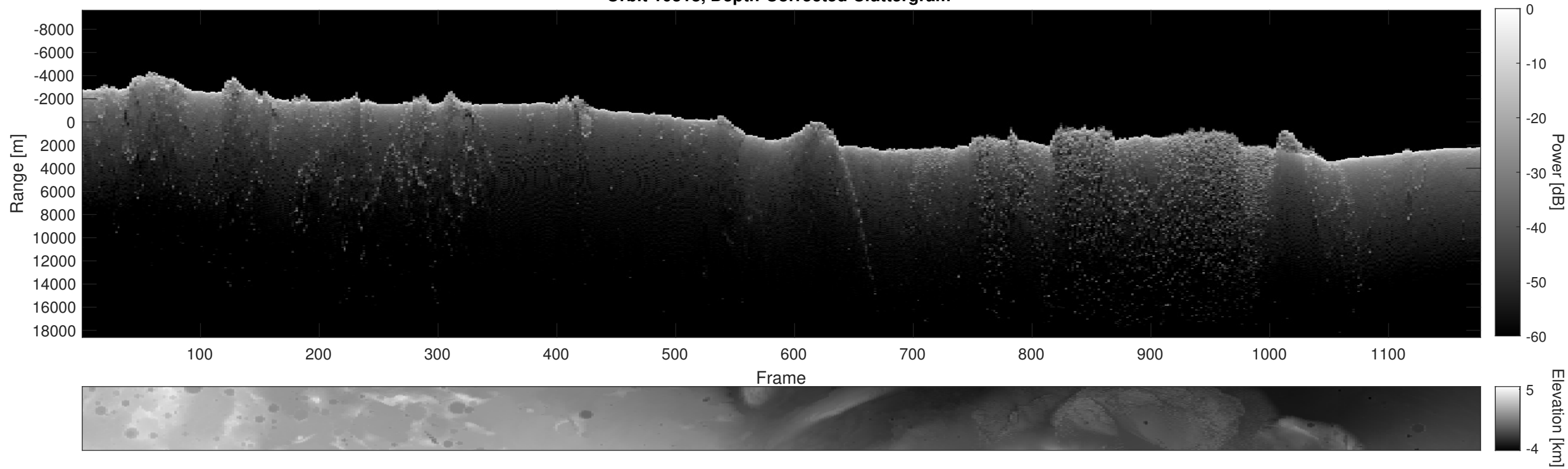
Orbit 10318, Depth-Corrected Cluttergram
