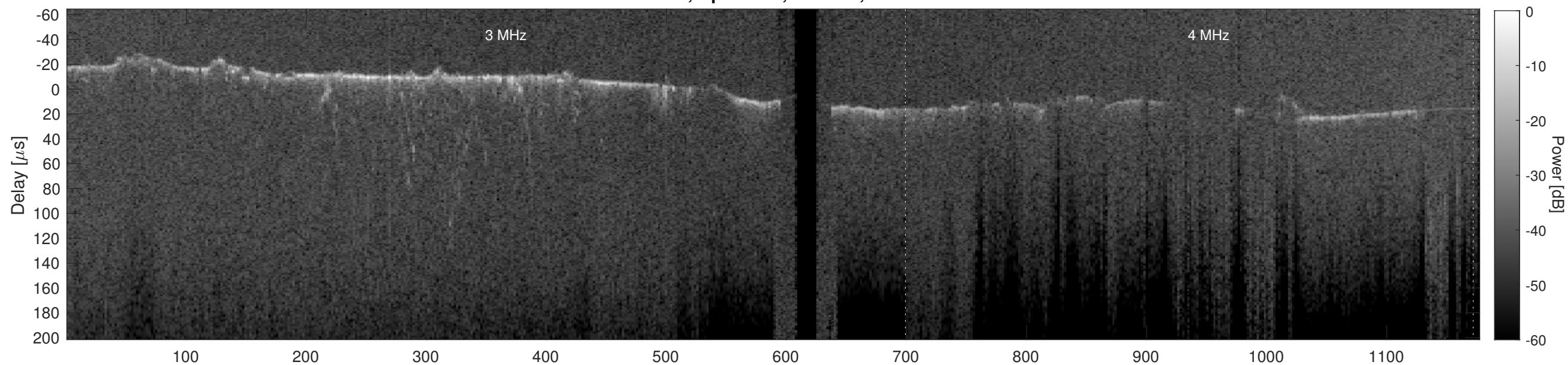
Orbit 10318, Cluttergram
