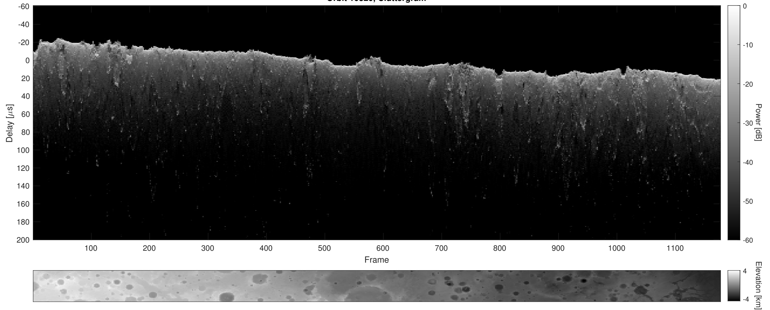
Orbit 10320, Cluttergram
