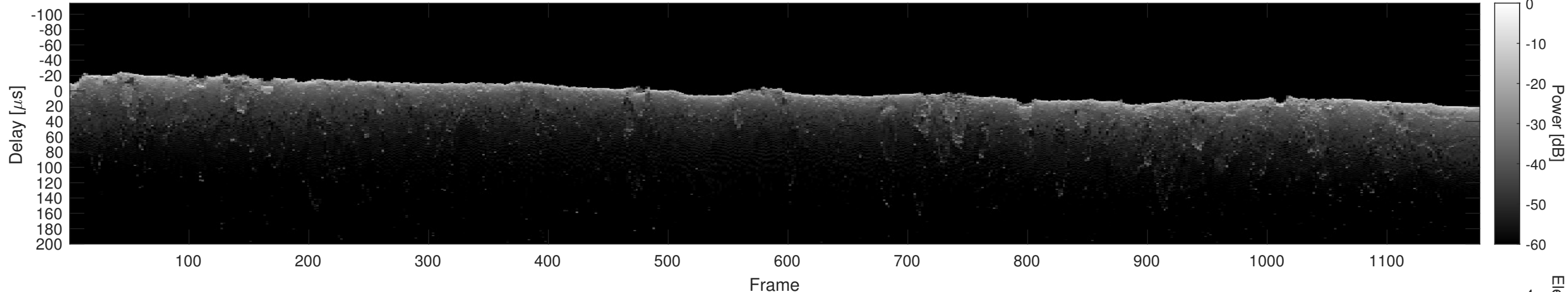
Orbit 10320, Cluttergram
