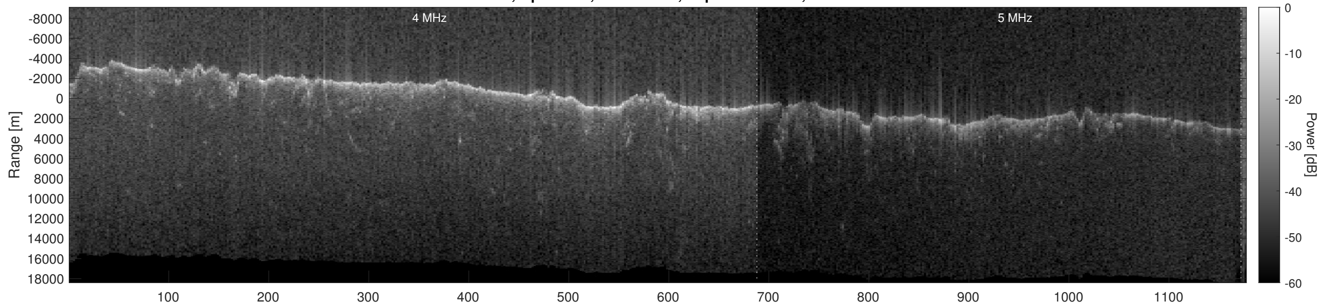
Orbit 10320, Optimized, No Window, Depth-Corrected, Channel 2
