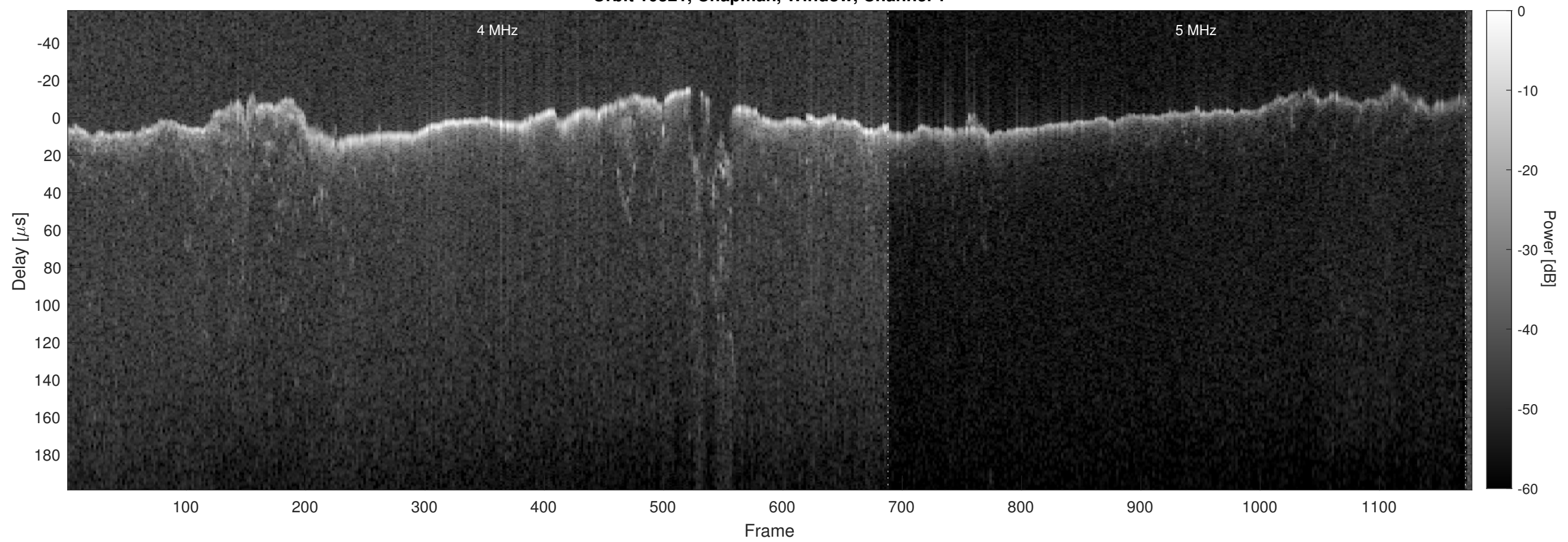
Orbit 10321, Chapman, Window, Channel 2
