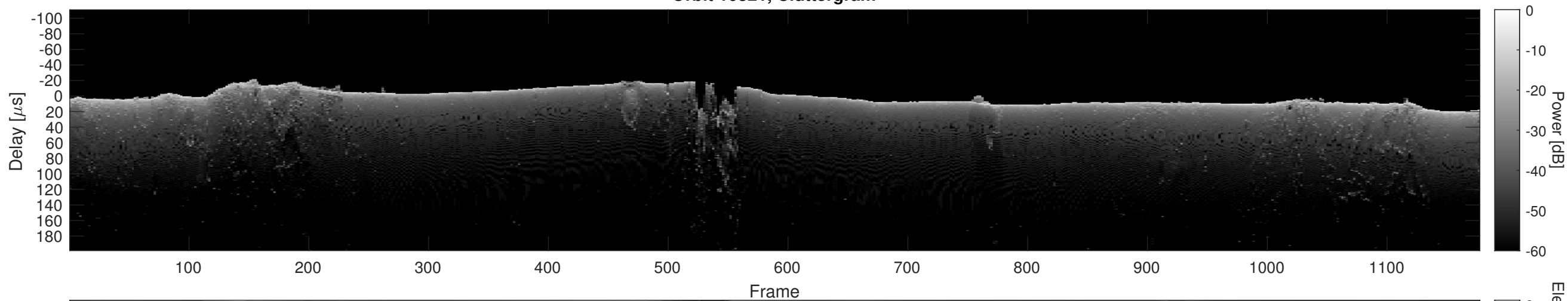
Orbit 10321, Cluttergram
