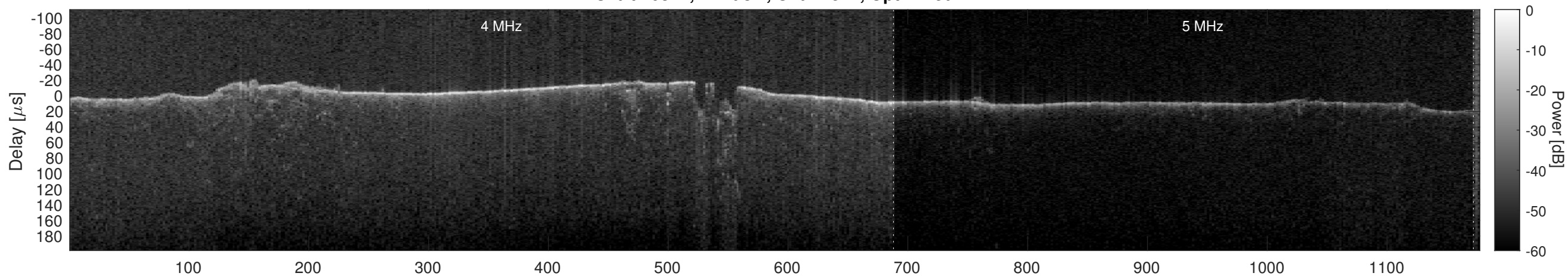
Orbit 10321, Cluttergram
