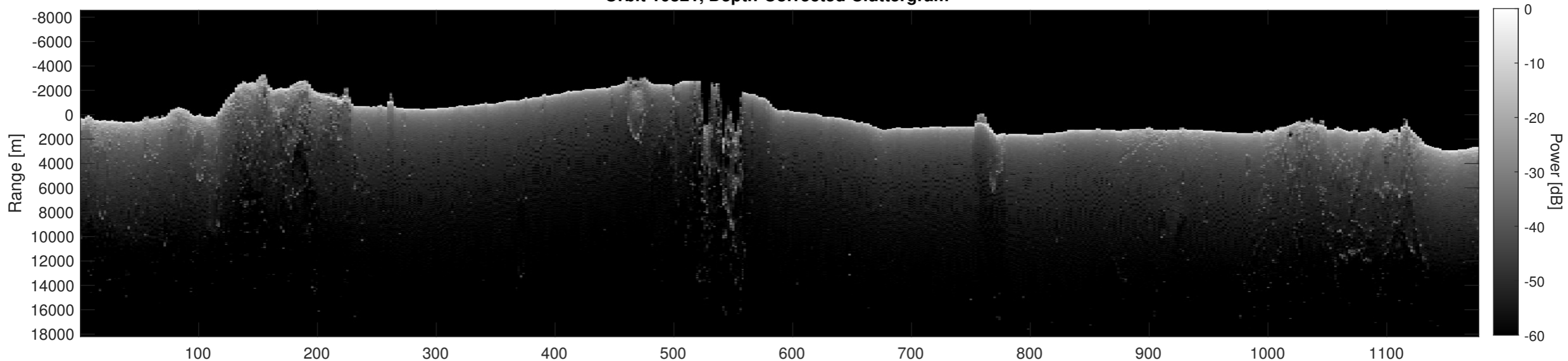
Orbit 10321, Depth-Corrected Cluttergram
