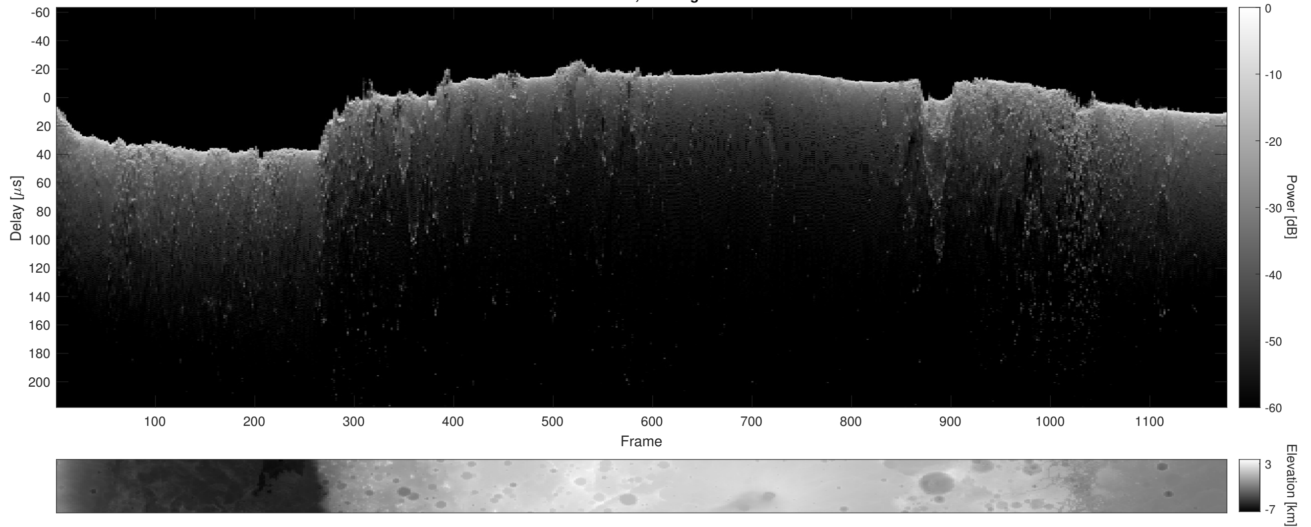
Orbit 10323, Cluttergram
