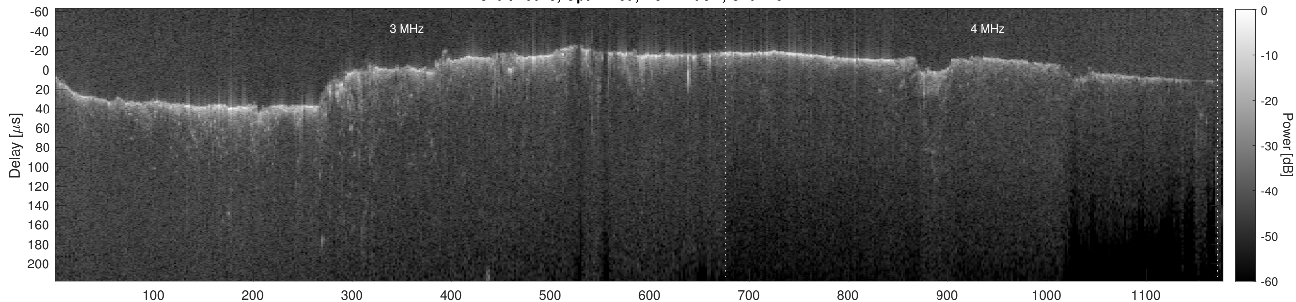
Orbit 10323, Cluttergram
