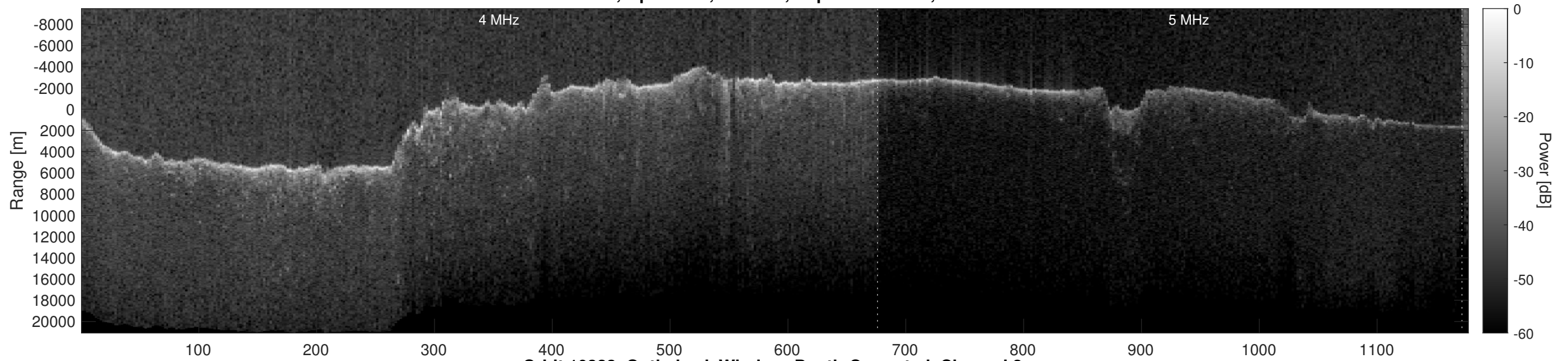
Orbit 10323, Optimized, Window, Depth-Corrected, Channel 2
