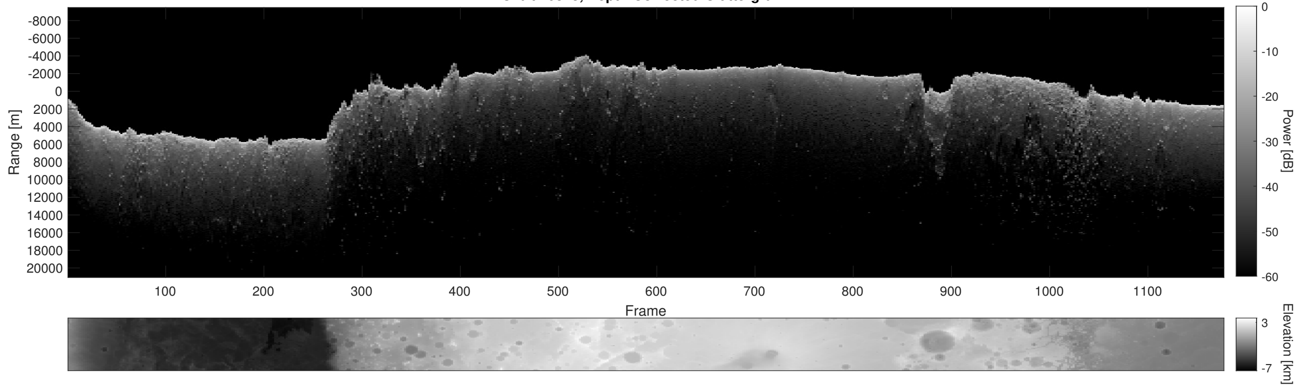
Orbit 10323, Depth-Corrected Cluttergram
