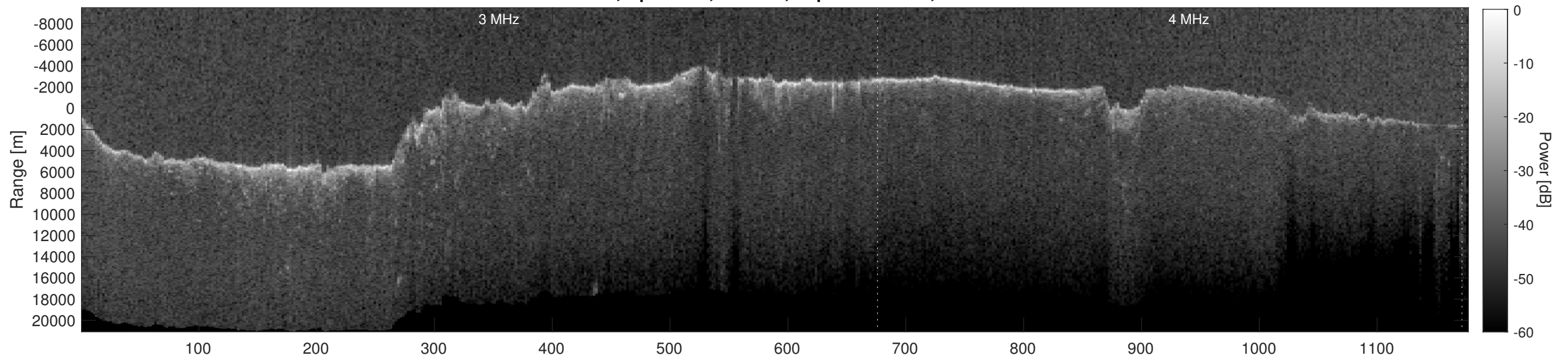
Orbit 10323, Depth-Corrected Cluttergram
