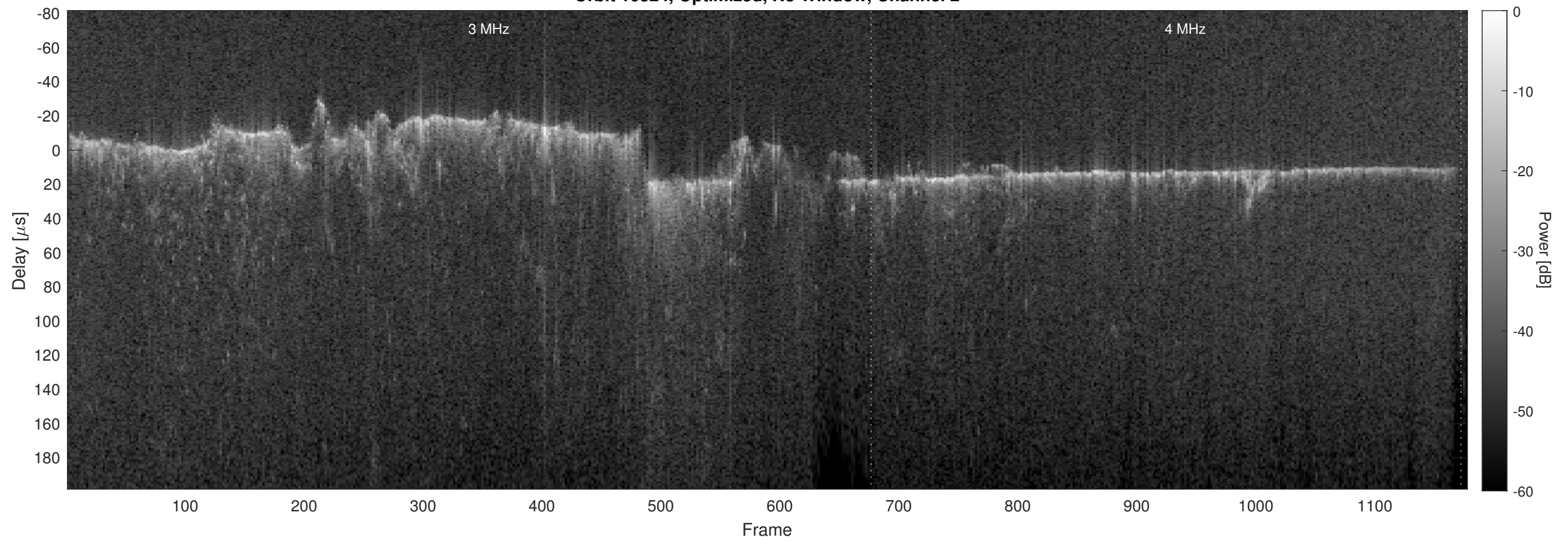
Orbit 10324, Optimized, No Window, Channel 2
