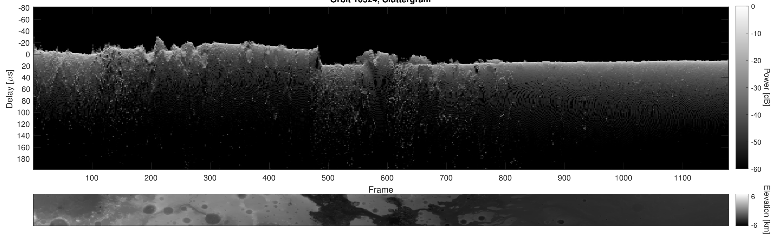
Orbit 10324, Cluttergram
