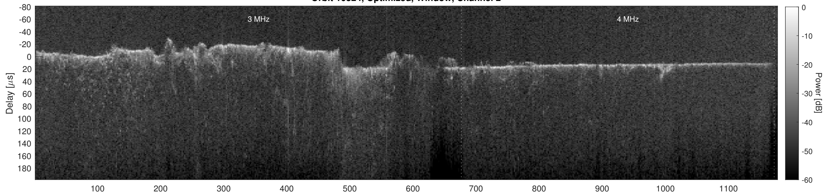
Orbit 10324, Cluttergram
