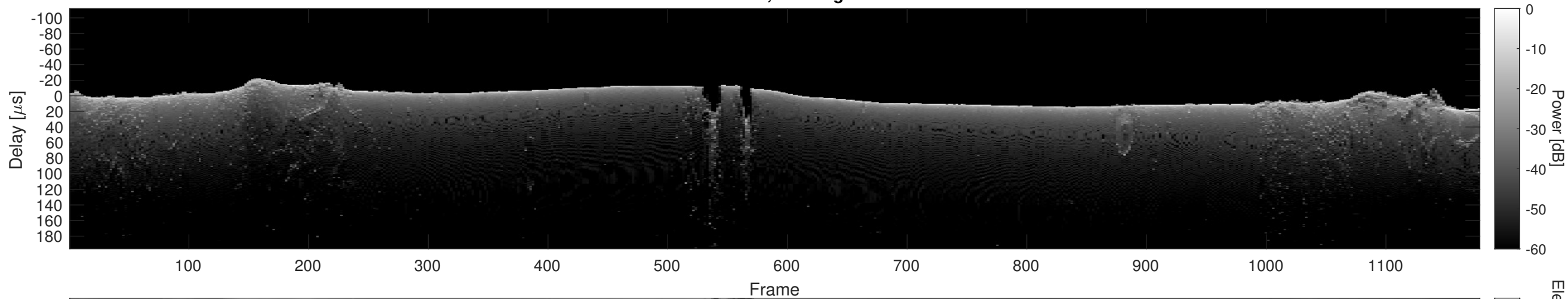
Orbit 10328, Cluttergram
