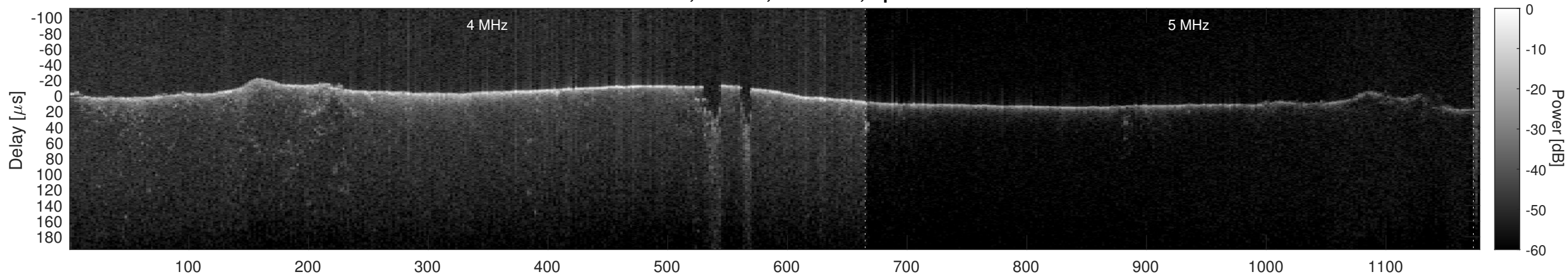
Orbit 10328, Cluttergram
