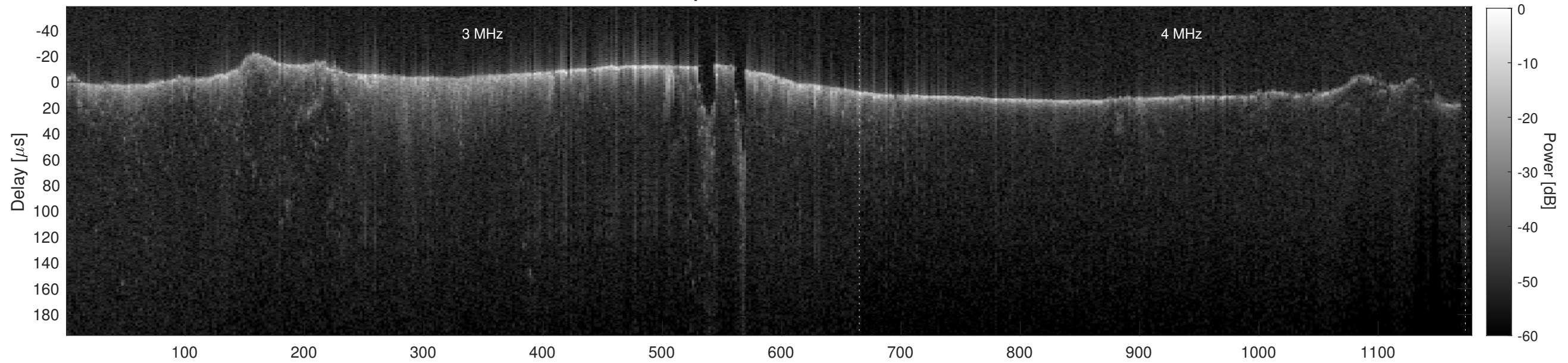
Orbit 10328, Cluttergram
