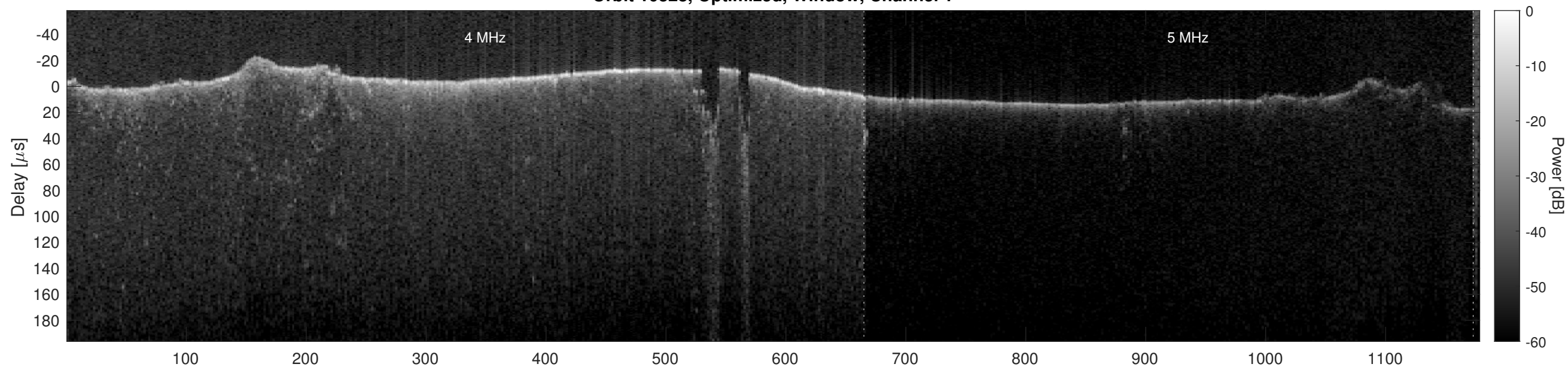
Orbit 10328, Optimized, Window, Channel 2
