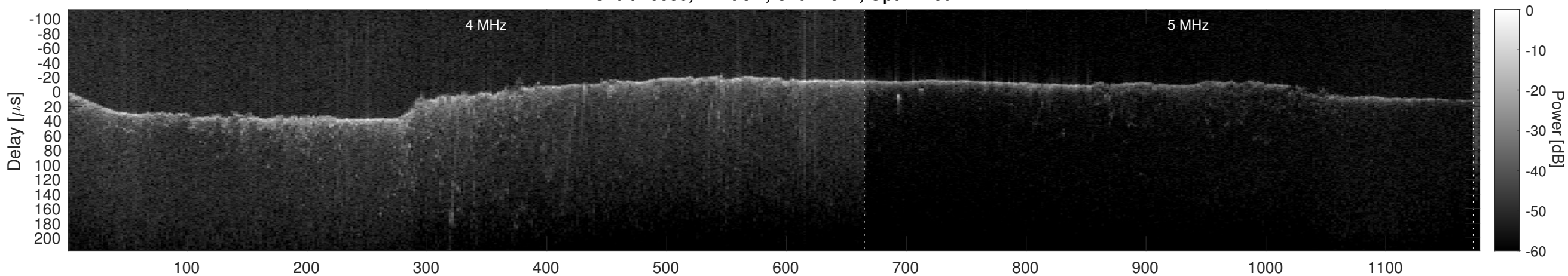
Orbit 10330, Cluttergram
