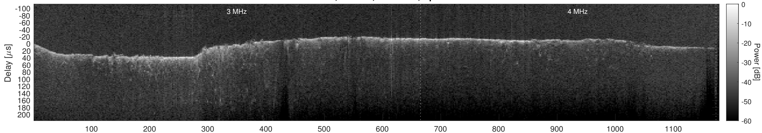
Orbit 10330, Cluttergram
