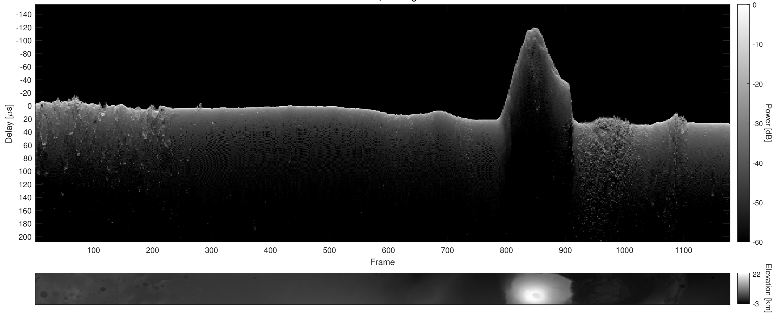
Orbit 10332, Cluttergram
