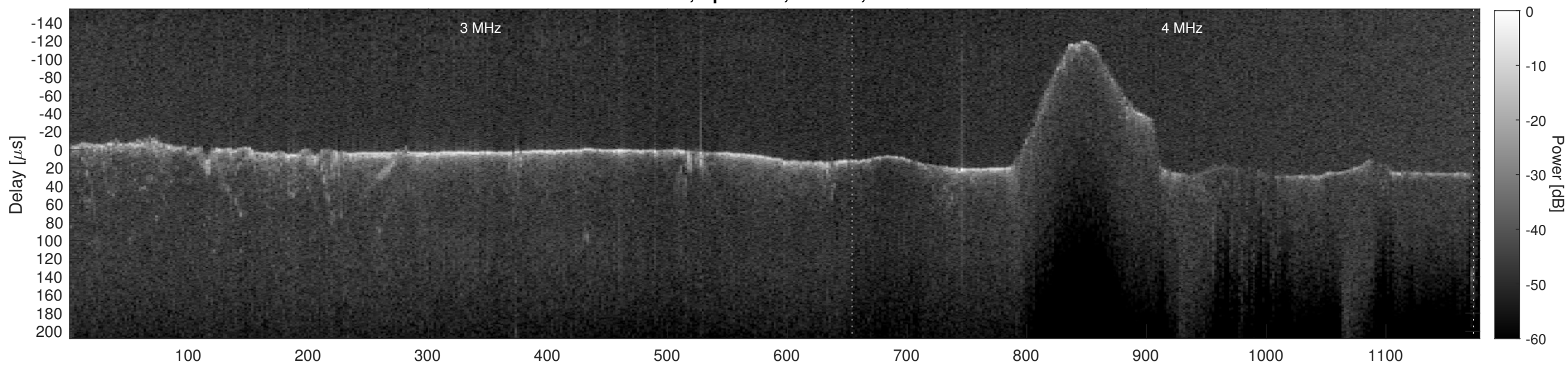
Orbit 10332, Cluttergram
