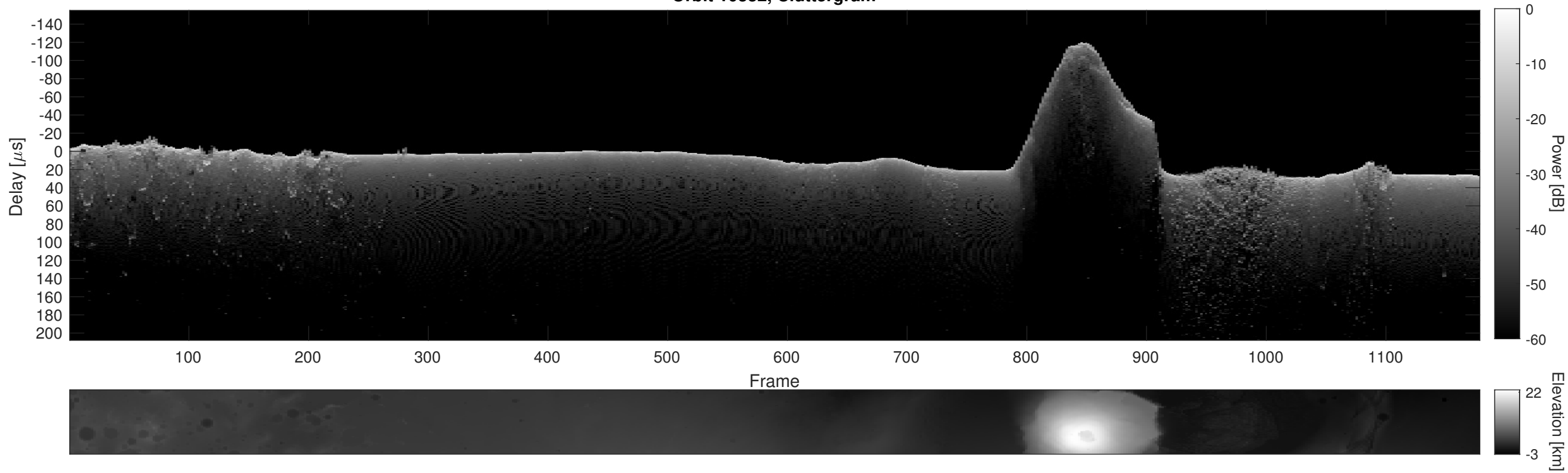
Orbit 10332, Cluttergram
