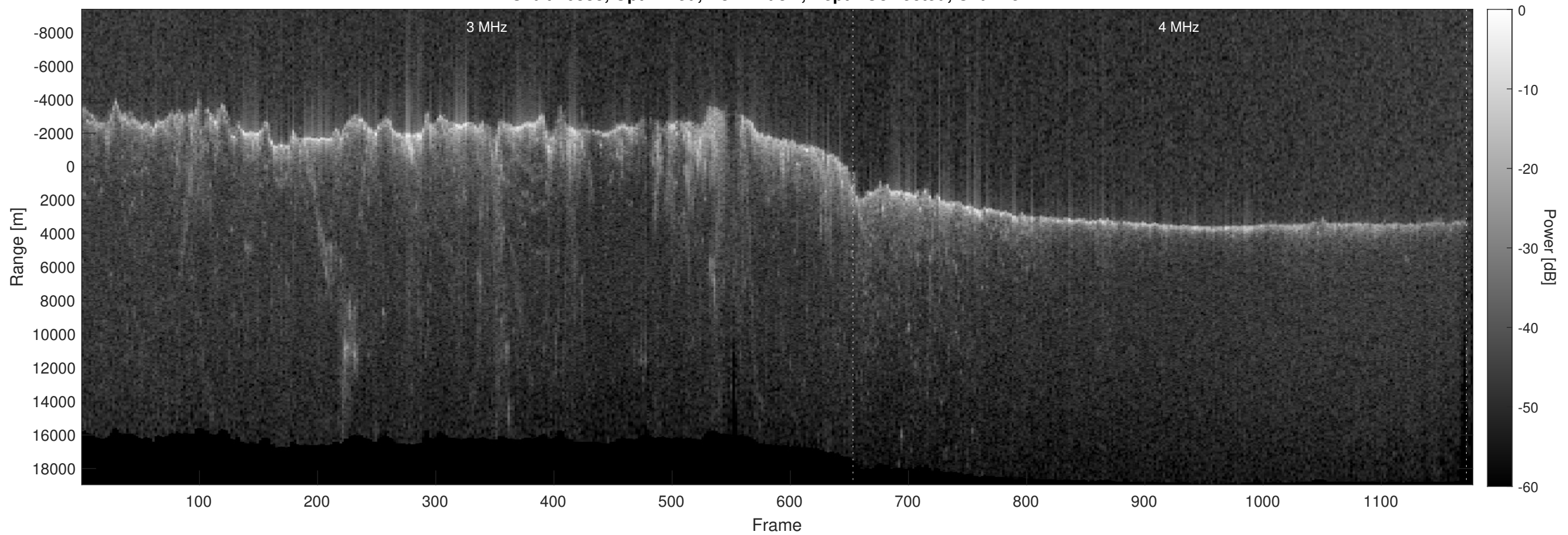
Orbit 10333, Optimized, No Window, Depth-Corrected, Channel 2
