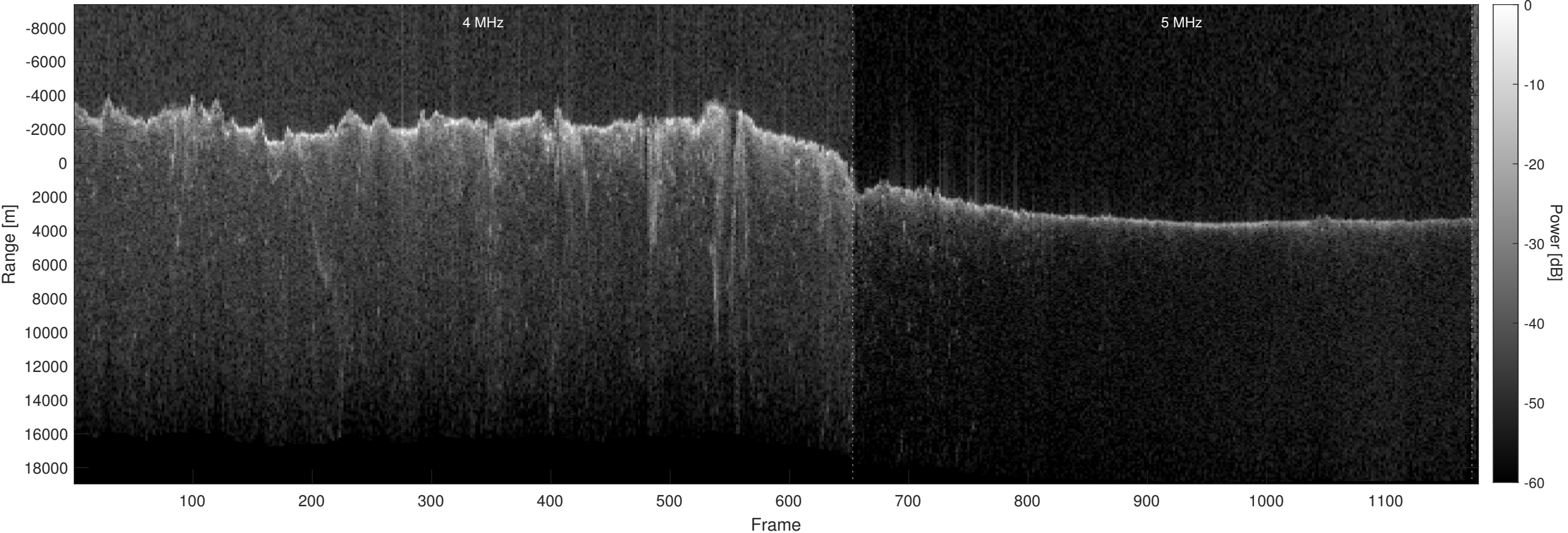
Orbit 10333, Optimized, Window, Depth-Corrected, Channel 2
