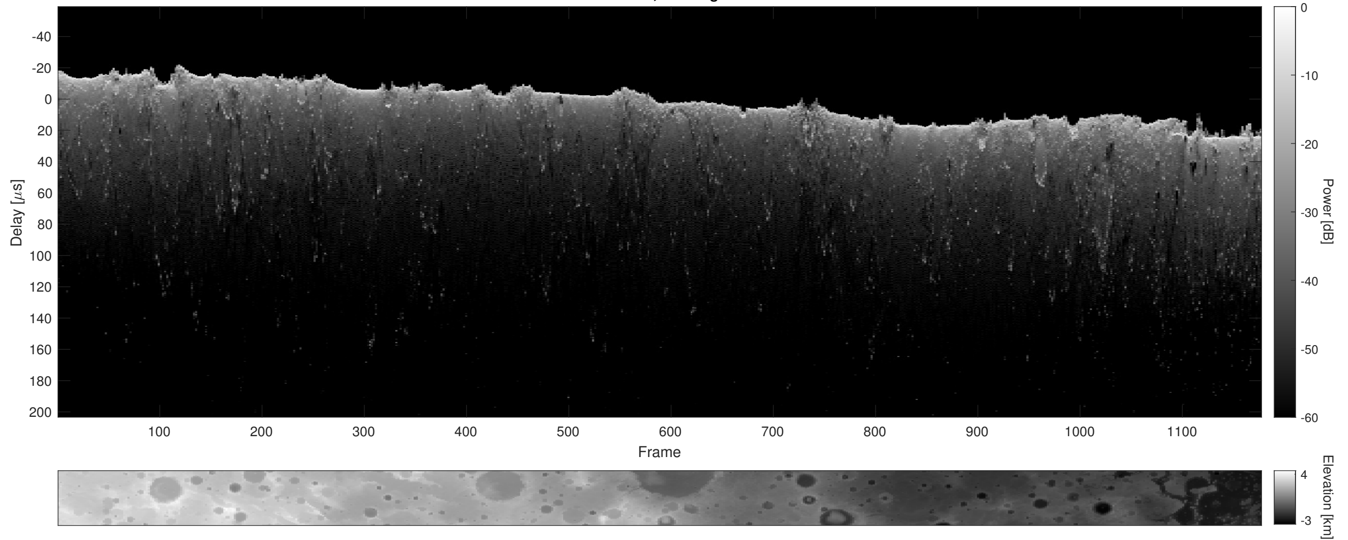
Orbit 10334, Cluttergram
