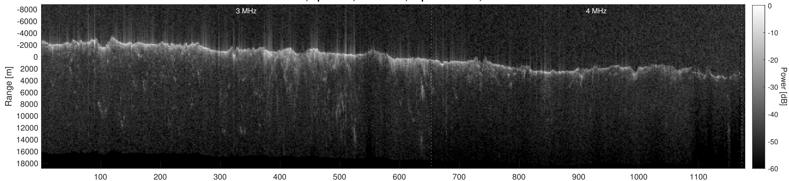
Orbit 10334, Depth-Corrected Cluttergram
