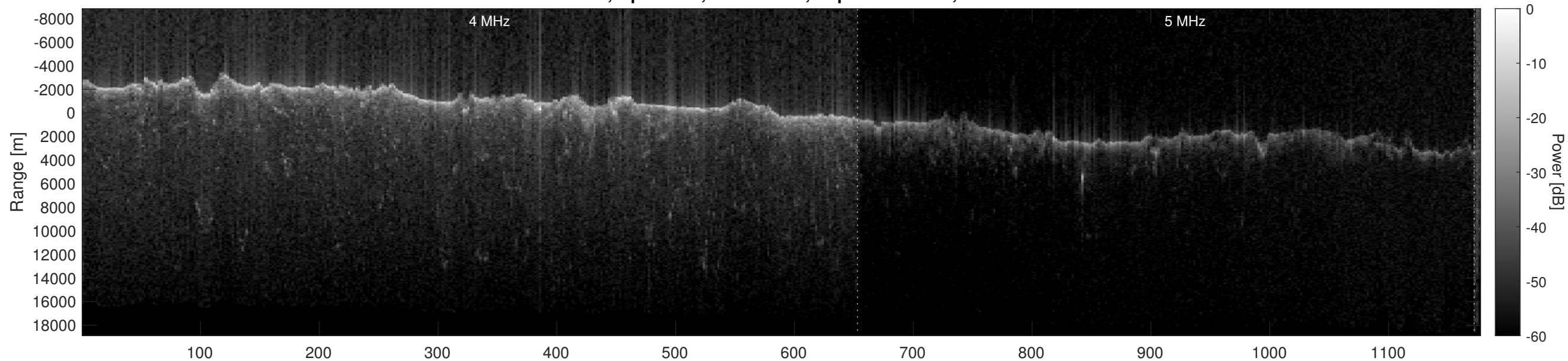
Orbit 10334, Optimized, No Window, Depth-Corrected, Channel 2
