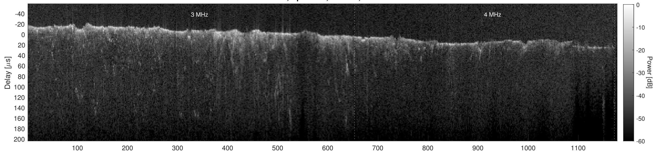
Orbit 10334, Cluttergram
