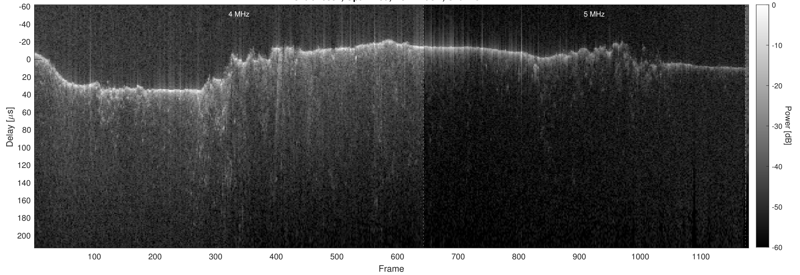
Orbit 10337, Optimized, No Window, Channel 2
