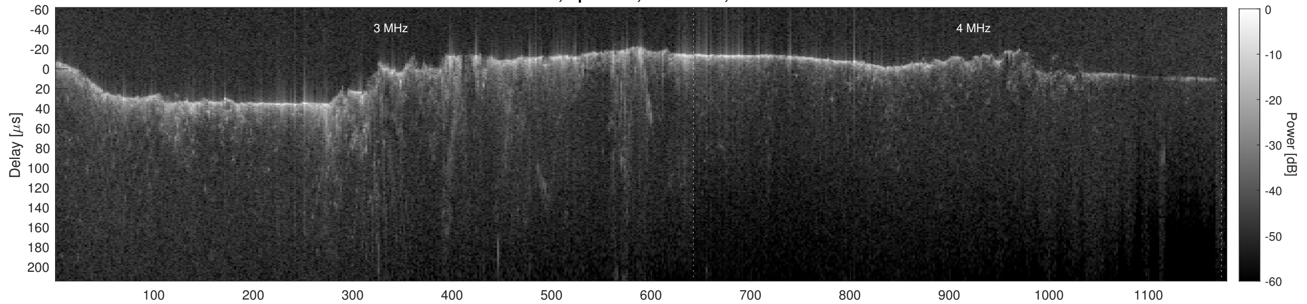
Orbit 10337, Cluttergram
